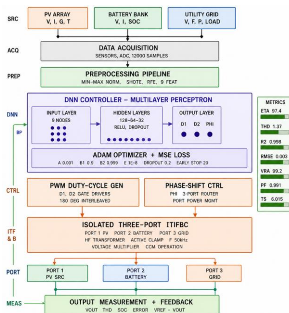
Figure 1. Proposed DNN-ITIFBCArchitecture
