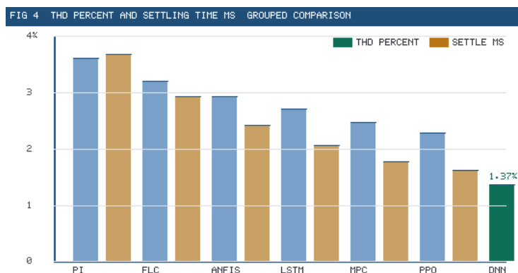
Figure 7. THD (%) and settling time (ms) grouped comparison. Teal/dark-orange = proposed (THD: 1.37%, t_s : 6.0 ms).
