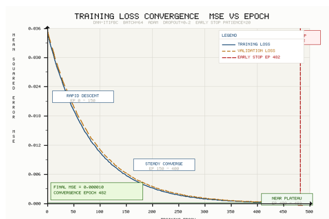
Figure 5. MSE loss convergence. Navy = training loss; orange dashed = validation loss; red = early stopping at epoch 482. Final MSE = 0.000010.
