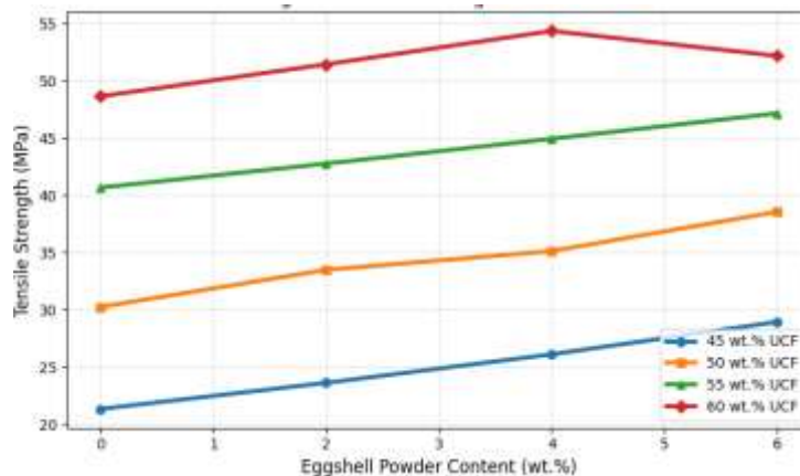
Fig.4.1 Tensile Strength Table 4 Output responses
