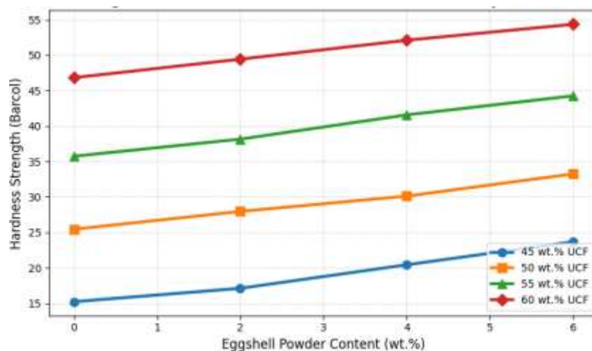
Fig.4.4 Hardness strength
