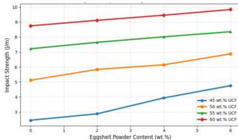
Fig.4.3 impact strengh
