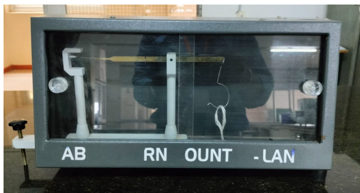
PLATE 3: BEESLEY BALANCE YARN COUNT TEST
