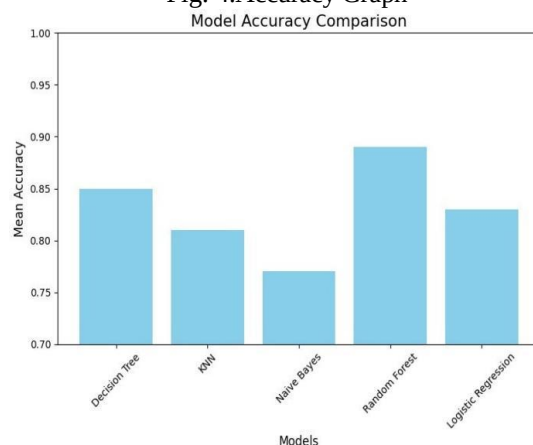
Fig. 4. Accuracy Graph
