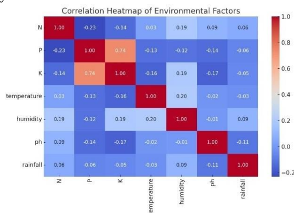
Fig.5.Heatgraph
