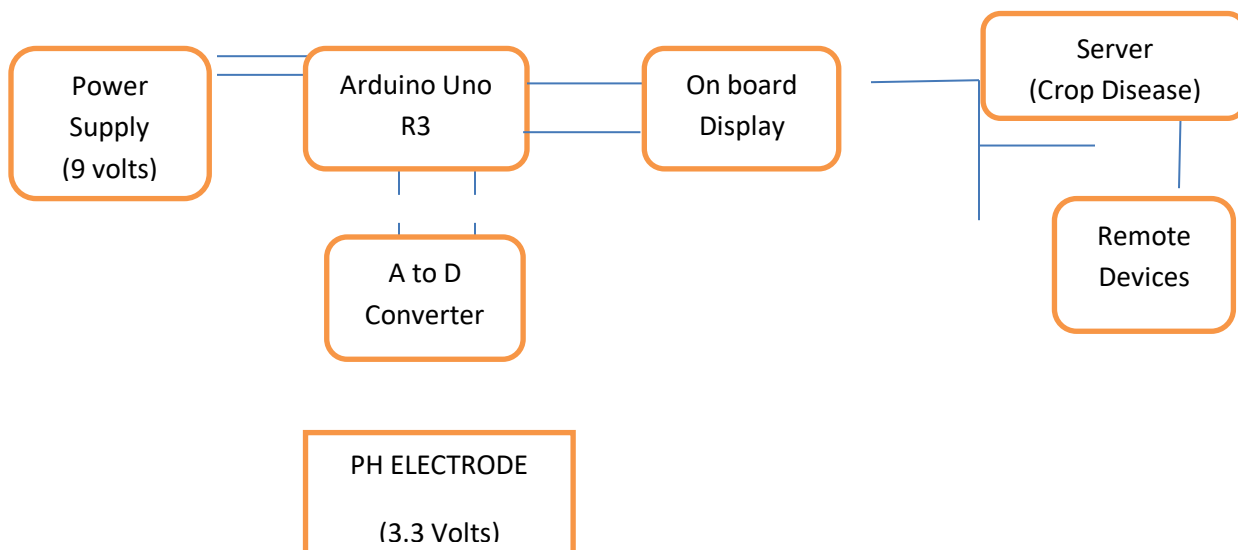
Figure 1: Block diagram of Soil Quality Analyzer and Crop Prediction System
