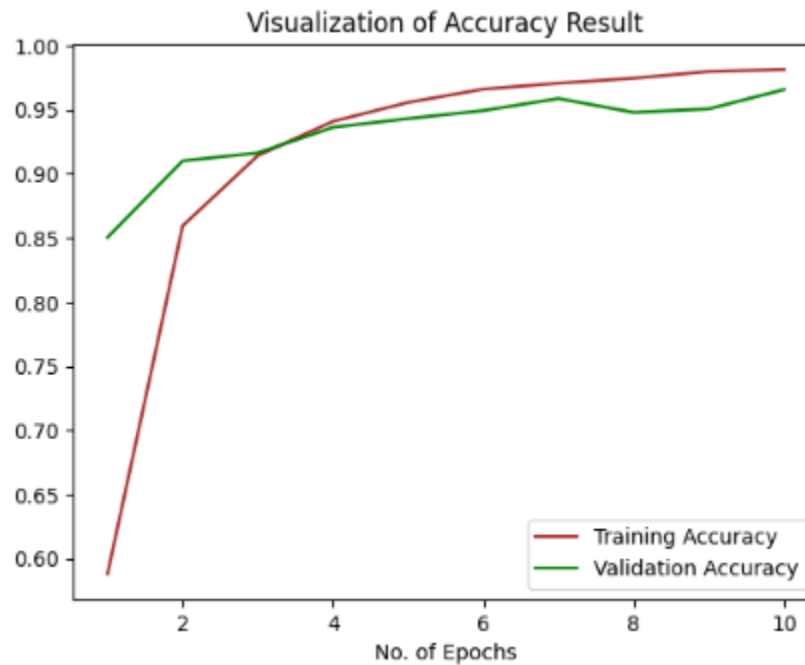
Figure 6.Accuracy Comparison Between Training and Validation Over Epochs
