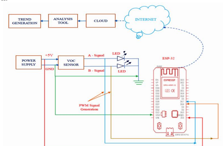
Figure. 4. Detailed Block Diagram of Acetone Detection
