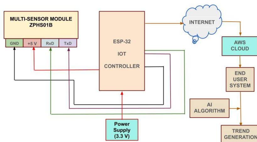
Figure. 1. Block Diagram - AcetoneMonitoring and Analysis System
